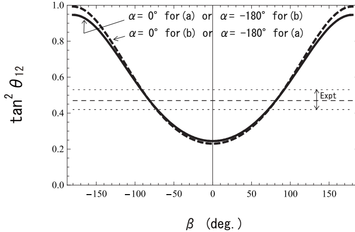
Fig. 3 Behavior of \tan^2 \theta_{12} versus \beta for typical values of \alpha . Curves are drawn by taking \alpha = 0^\circ and -180^\circ for inputs (a) (s_\delta, s_1, s_2, s_3) = (+1, -0.2255, -0.0376, -0.0174) and (b) (s_\delta, s_1, s_2, s_3) = (+1, -0.2255, +0.0376, +0.0174) , where s_\delta = \sin \delta_{KM} .
